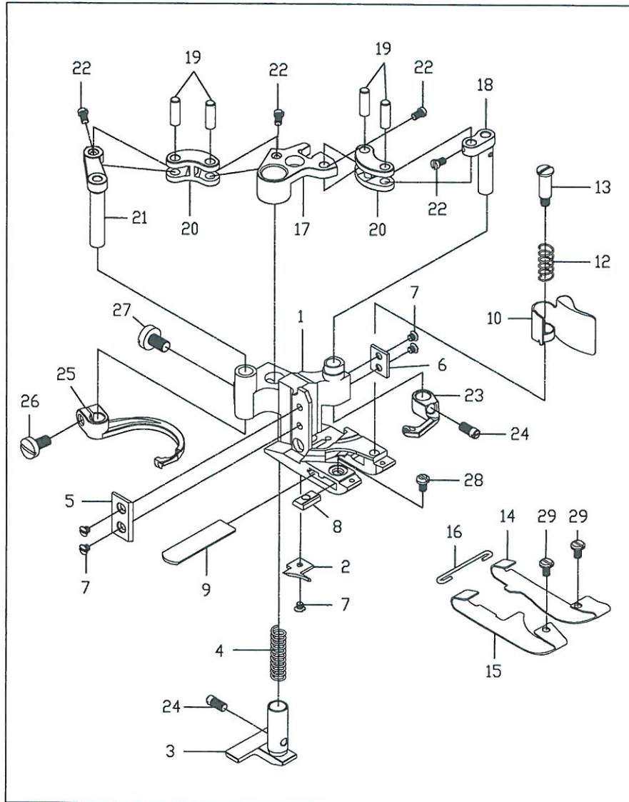
NTD6712-H5/H6(雙切)
