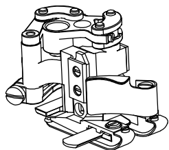
NTD6703D-M(雙切)
